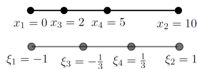
Figure 3: Third order element for 1D problems.
