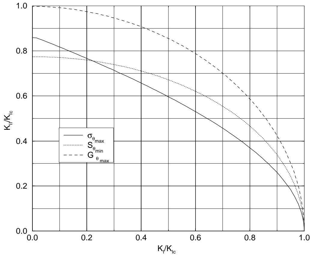
Figure 10.5: Locus of Fracture Diagram Under Mixed Mode Loading
