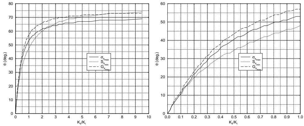
Figure 10.4: Angle of Crack Propagation Under Mixed Mode Loading
